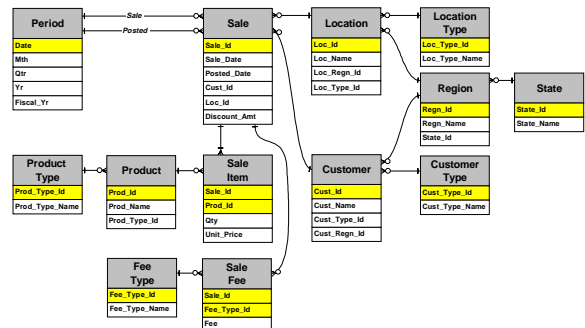
Figure 5. Example Data Model
