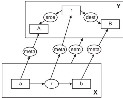
Figure 8. Fundamental Relations Between a Space X and a Meta-Space Y.
